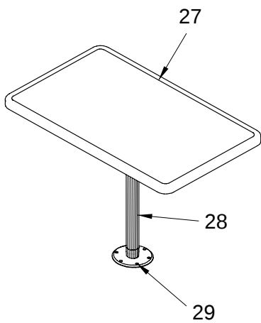
COCKPIT TABLE
