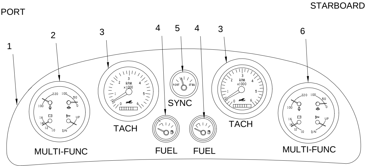
INSTRUMENT PANEL ( STERN DRIVE)
